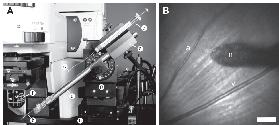
Fig. 2. A) Photograph of the micro-advancer. The device is clamped to a micromanipulator, which is attached to a movable microscope stage. A Hamilton syringe is clamped to the syringe holder and is connected to the injection needle by PE-10 tubing. a, micro-advancer; b, guard needle; c, PE-10 tubing; d, Hamilton syringe; e, syringe holder; f, microscope objective lens; g, micromanipulator; h, microscope stage. B) Reflected light confocal image of the retina, showing the tip of the micro-advancer injection needle (n), an arteriole (a) and a venule (v). Scale bar, 250 \mu m.
