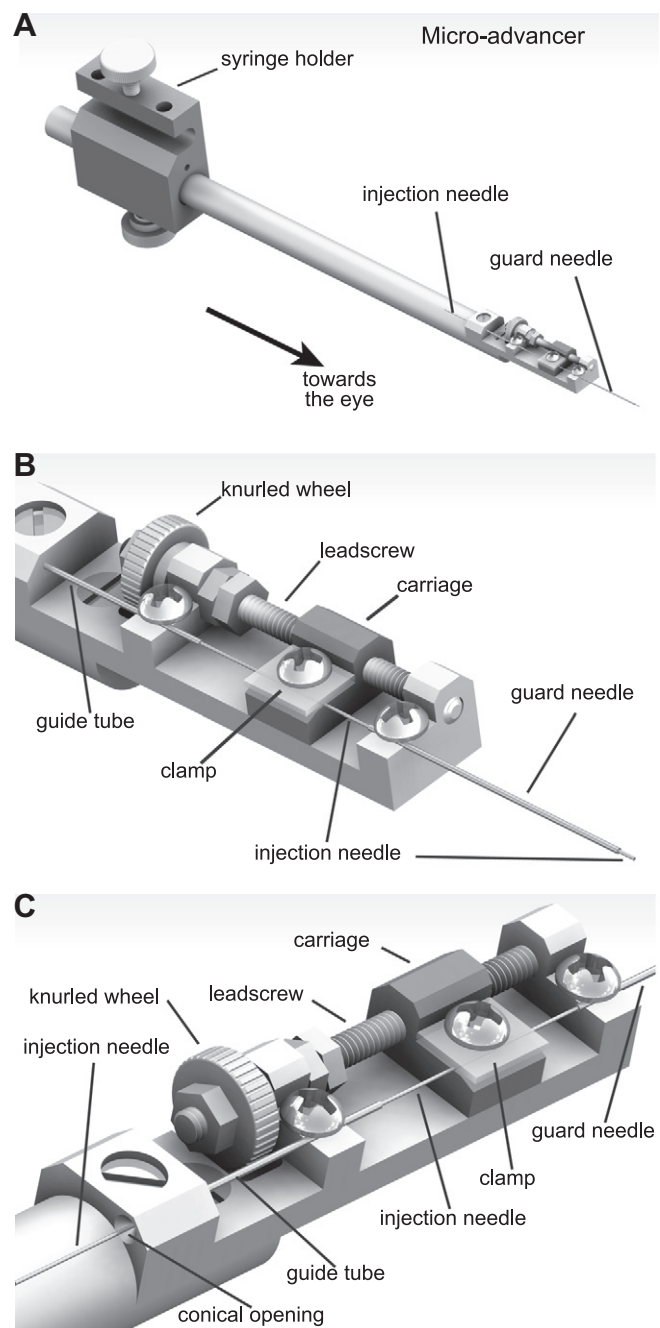
Fig. 1. Three-dimensional drawings of the micro-advancer, with components labeled. A) Overview of the micro-advancer, with the end of the device pointing toward the eye at the right. B) Close-up of the micro-advancer mechanism at the end of the device nearest the eye. C) Close-up of the micro-advancer mechanism, viewed from a different angle. The 3-D drawings were rendered using ViaCAD Pro v7.0 (Encore Software). Computer-aided design drawings of the device are provided in the Supplemental material .
